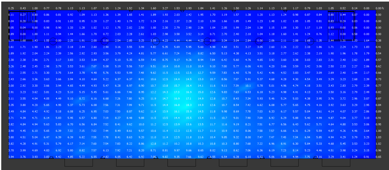
Figure 4. Light Plot with proposed new lighting (Courtesy of Craft Metal Products)
